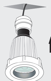
(F) Fix Lamp Holder, Lamp and Bezel
