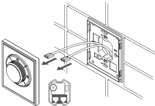
3. Plug in the RJ45 connectors.
