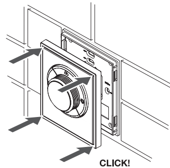
4. Push and clip the main unit back into the base.
