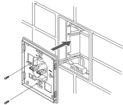
2. Mount base to a standard (UK, EU, USA, JP) switch box.
