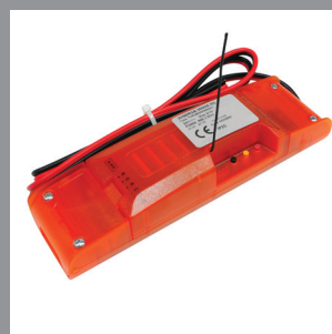
master 12V/24V 150W/300W WISERGB STRIP M3
