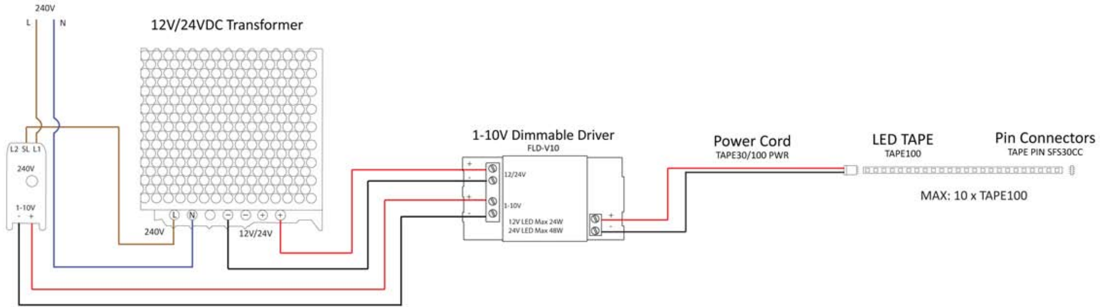
1-10V DIMMER MODULE DPD10VDCMB
