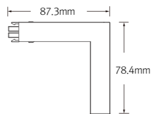
* LED 90° Connector NDF3 40K-230V-C90-90
