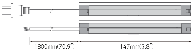
* LED Power Cord NDF3 40K-230V-C90-FF-PC / OPC
