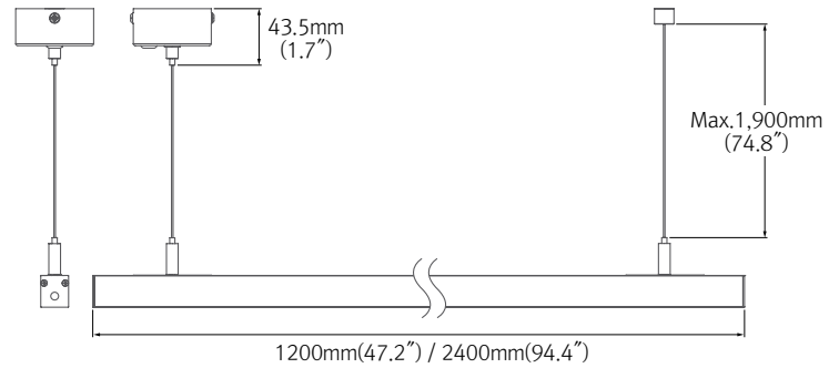
* NDF Extrusion Line
