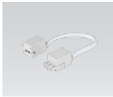
Connecting Cable __NDFPTC/T (150mm) __NDFPTC1/T (300mm) __NDFPTC2/T (600mm) __NDFPTC4/T (1,200mm) __NDFPTC6/T (1,800mm)
